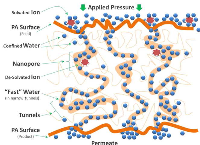
Fig. 7. Schematic summarizing some of the key features of semipermeable PA membrane materials that have emerged from molecular modeling studies in recent years. The membrane is a dynamic polymer network that continually vibrates and alters its conformation around some “ergodic” or time-average structure. Thus, although they are quasi-stable, transmembrane tunnels and nanoporous regions can form and decay depending on local solvation and ion interactions. Depending on tunnel dimensions and composition, water molecules placed under a driving pressure may exhibit anomalous “fast” transport kinetics, referred to by Gao and co-workers [30] as “flush” diffusion. Extensively hydrogen-bonded “continuum” or clustered water, resembling that of bulk water in terms of its density and diffusion properties, primarily exists inside the membrane in expanded nanopores. Both water and solutes appear to transit the membrane via a jump or hopping mechanism in which the frequency of jumps controls the water production rate ( i.e. , membrane flux).
