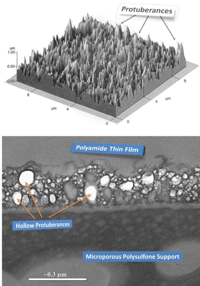
Fig. 2. AFM and TEM images of polyamide TFC membranes showing rough surface morphology and hollow protuberances (unpublished images provided courtesy of Bob Riley, Separation Systems Technology, San Diego, California, USA). The structural variations seen in the PA discriminating layer make it challenging to know what area to model.
