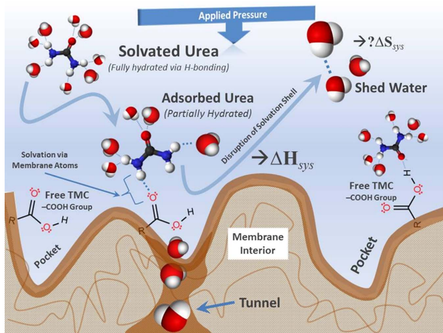
Fig. 4. Schematic illustrating the effects of shedding of solvation water in the adsorption of potential organic foulants to PA membranes. This basic mechanism, and variations of it, have been discussed in the publications of Hughes and Gale [58] and Shen et al. [48]. Here the rough membrane surface is represented by the thick wavy horizontal line (light brown), with the feed solution above the line (blue background) and the membrane network lying below (brown). Organic compounds having stronger ( i.e. , tightly bound) hydration shells due to increased hydrogen-bonding interactions, such as urea (shown), are forced to shed waters of solvation at a larger thermodynamic penalty ( -\Delta H_{sys} ) compared to those with weaker shells as they approach and undergo binding to the membrane surface. The shed water molecules contribute to complex changes in the system entropy ( -\Delta S_{sys} ), which presumably increases due to release from the organic solvation shell, but also decreases due to hydrogen-bonding interactions with the bulk water phase. (For interpretation of the references to color in this figure legend, the reader is referred to the web version of this article).
