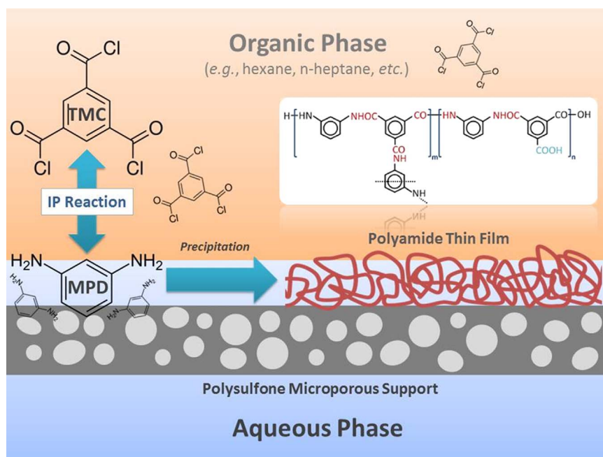
Fig. 1. Schematic of general synthesis protocol for preparation of the “Cadotte” polyamide TFC membrane. TMC and MPD residues undergo interfacial polymerization at an organic/aqueous interface leading to precipitation of a thin insoluble PA film on the surface of a microporous polysulfone structural support.
