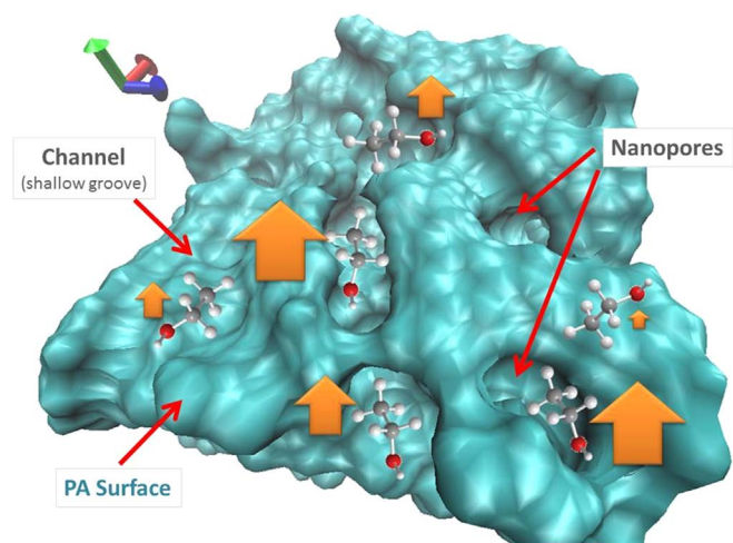
Fig. 5. Concept of ligand (solute or foulant) binding to a morphologically heterogeneous PA membrane surface exhibiting an uneven landscape. See text for details. The hypothetical PA surface is rendered as a Connolly probe surface (probe diameter=1.4 Å). Small ligands or foulant molecules, such as ethanol shown in this instance, may undergo strong or weak binding depending on where adsorption takes place. Adsorption within deep nanopores or grooves have the potential to strengthen binding by maximizing the number of attractive intermolecular interactions. In the diagram, strong ethanol binding is illustrated by the larger orange-colored arrows; weaker binding by smaller arrows.
